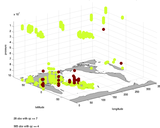
RADIOSONDE_U_WIND_COMPONENT level (10000.00 - 97770.00) 01-Aug-2006 03:00:01 - 01-Aug-2006 09:00:00 NCEP BUFR observation (993 bad observations)
